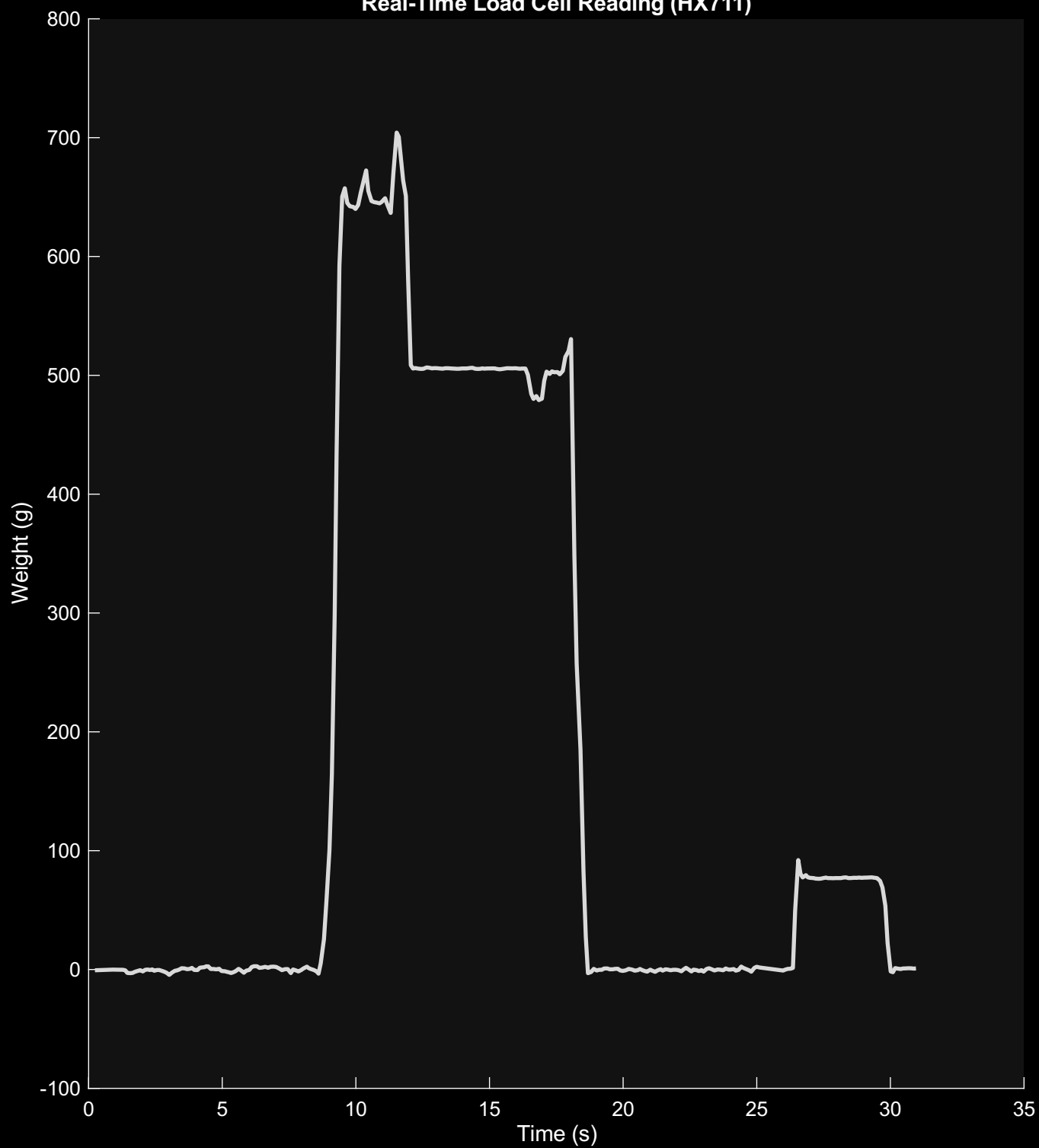
Real-Time Load Cell Reading (HX711)
